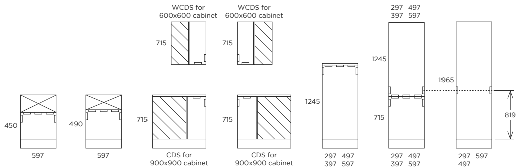
Ceramic Sink Configurations
