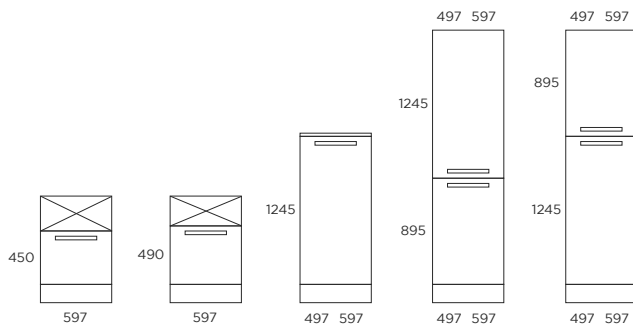
Ceramic Sink Configurations
